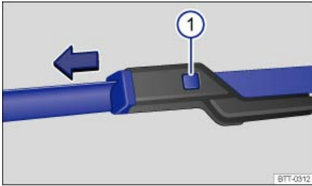
Fig. 162 Changing the windshield wiper blades.
