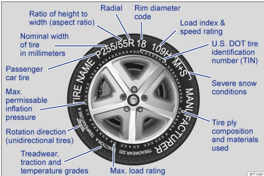
Fig. 107 International tire labeling.
