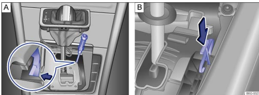
Fig. 172 Releasing the selector lever lock (versions A and B).
