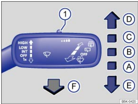
Fig. 81 Operating the front windshield wipers.
