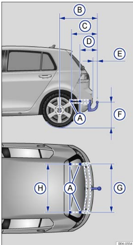
Fig. 101 Dimensions and attachment points for retrofitting a trailer hitch.
