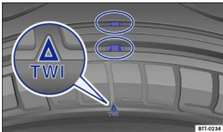
Fig. 104 Tread pattern: Wear indicator.
