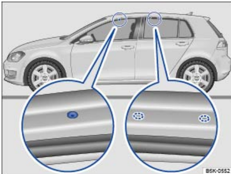
Fig. 99 Mounting points for the base carrier and roof rack on 4-door vehicles.
