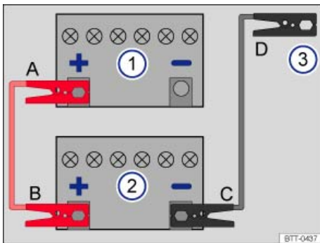
Fig. 189 Diagram for attaching the jumper cables: Dead battery 1 and booster battery 2.
