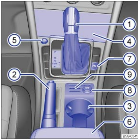
Fig. 7 Overview of the lower center console.
