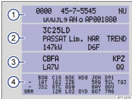
Fig. 17 Vehicle identification label: Shown in the example with engine identification code CBFA 3.
