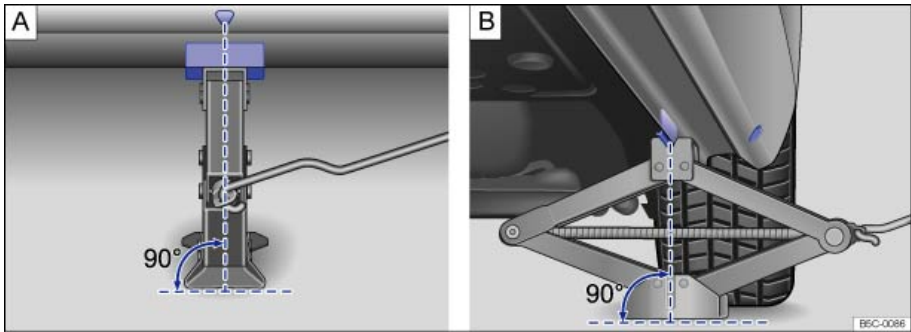
Fig. 181 Jack in position at the left rear lift point.
