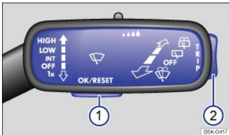
Fig. 14 On the right side of the steering column (vehicles without a multi-function steering wheel): Windshield wiper lever with controls for instrument cluster menus and displays.
