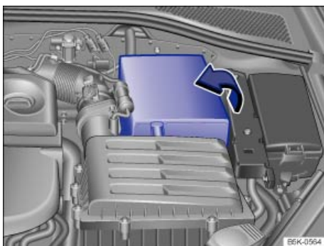
Fig. 161 In the engine compartment: Open the sleeve covering of the vehicle battery.
